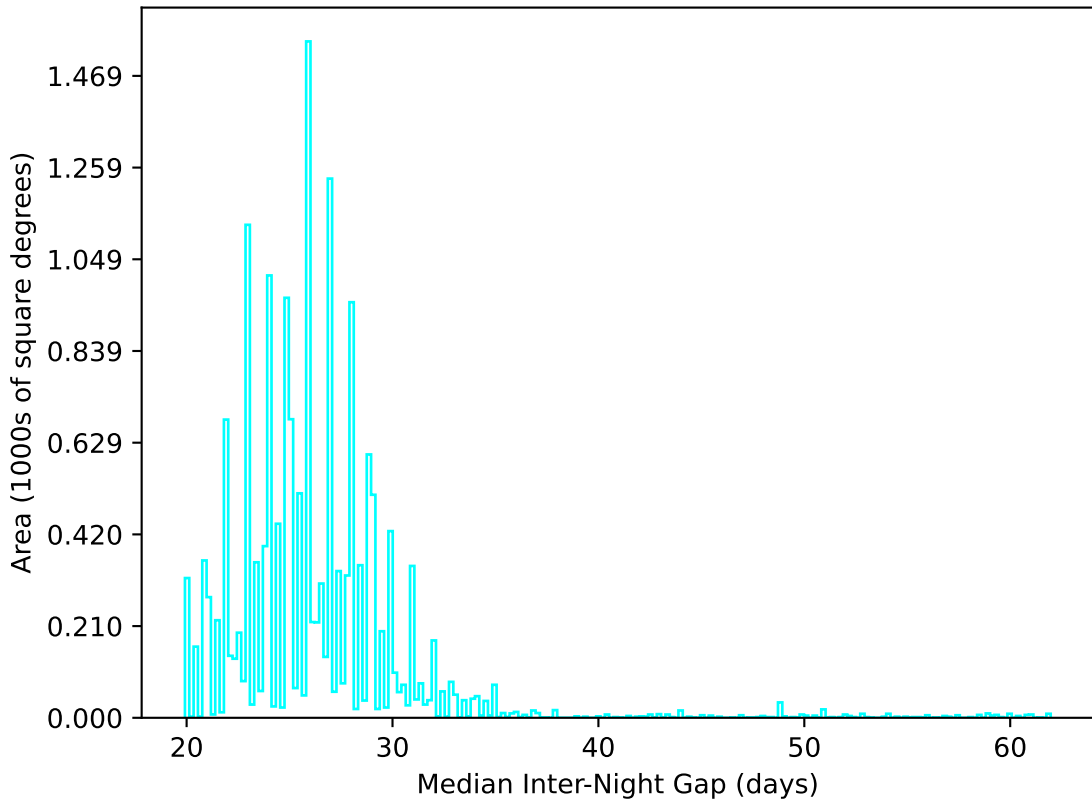
too_elab_r16_d3_ugrizy_v3.4_10yrs WFD u band: Median Inter-Night Gap
