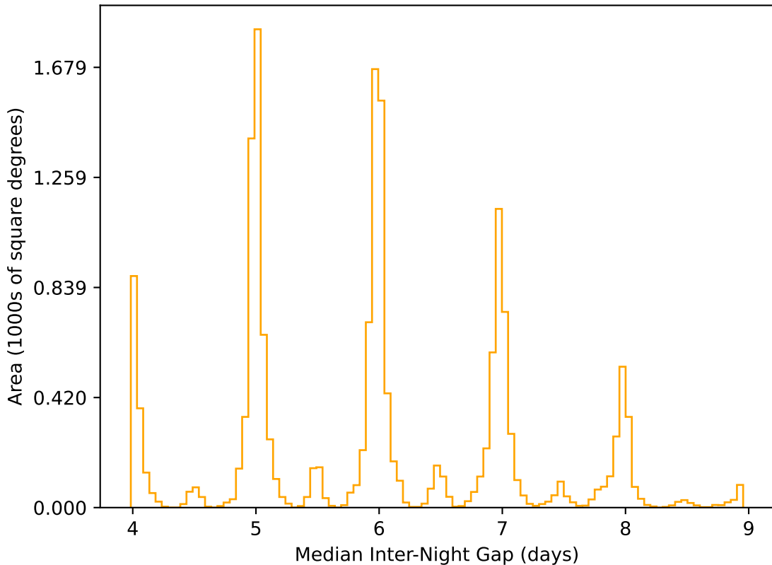
too_elab_r16_d3_ugrizy_v3.4_10yrs WFD r band: Median Inter-Night Gap
