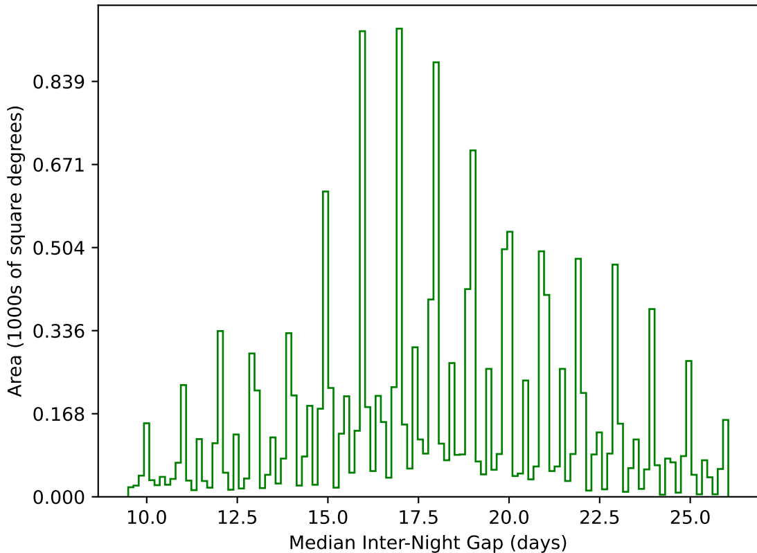
too_elab_r16_d3_ugrizy_v3.4_10yrs WFD g band: Median Inter-Night Gap
