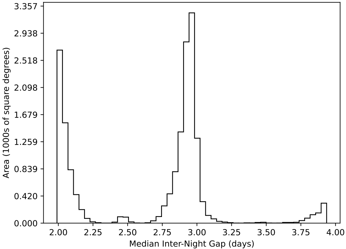
too_elab_r16_d3_ugrizy_v3.4_10yrs WFD all bands: Median Inter-Night Gap
