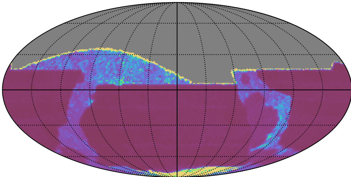
too_elab_r16_d3_ugrizy_v3.4_10yrs All sky z band: Median Inter-Night Gap
