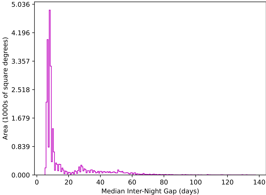
too_elab_r16_d3_ugrizy_v3.4_10yrs All sky z band: Median Inter-Night Gap
