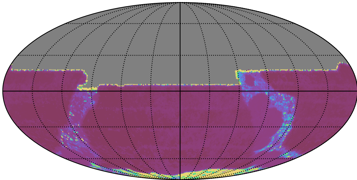
too_elab_r16_d3_ugrizy_v3.4_10yrs All sky y band: Median Inter-Night Gap
