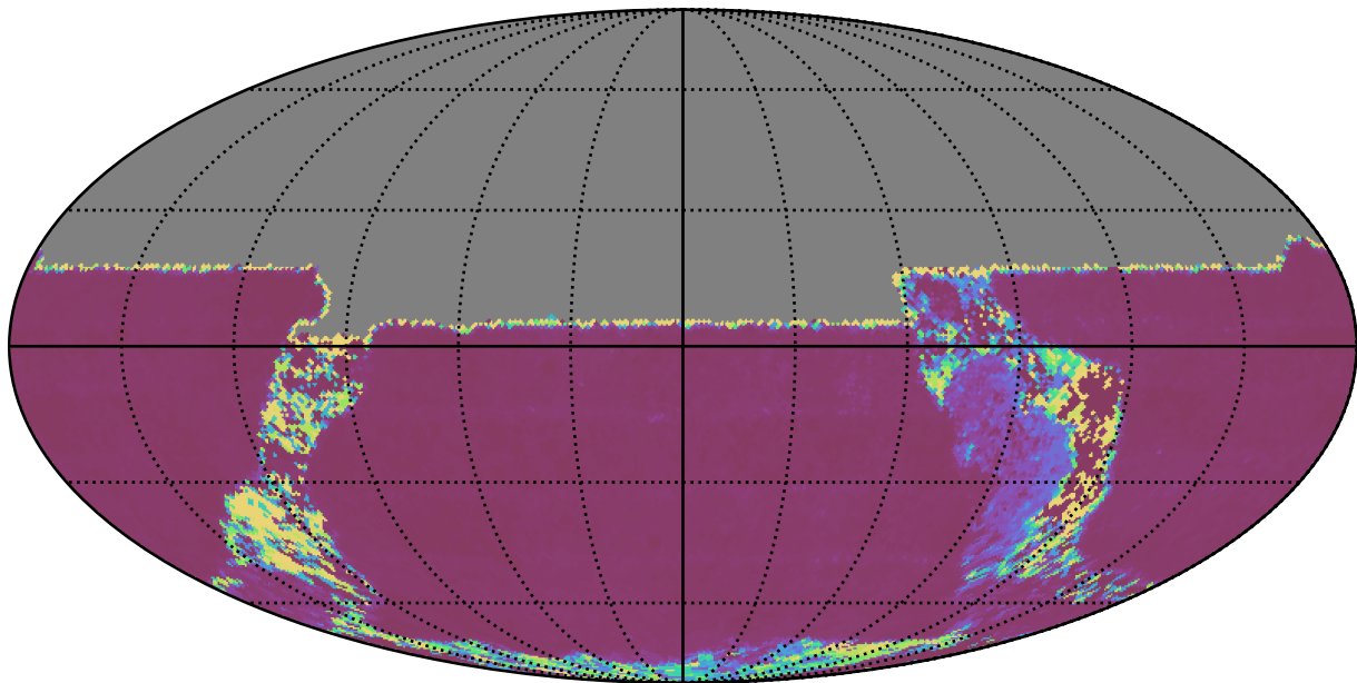
too_elab_r16_d3_ugrizy_v3.4_10yrs All sky u band: Median Inter-Night Gap
