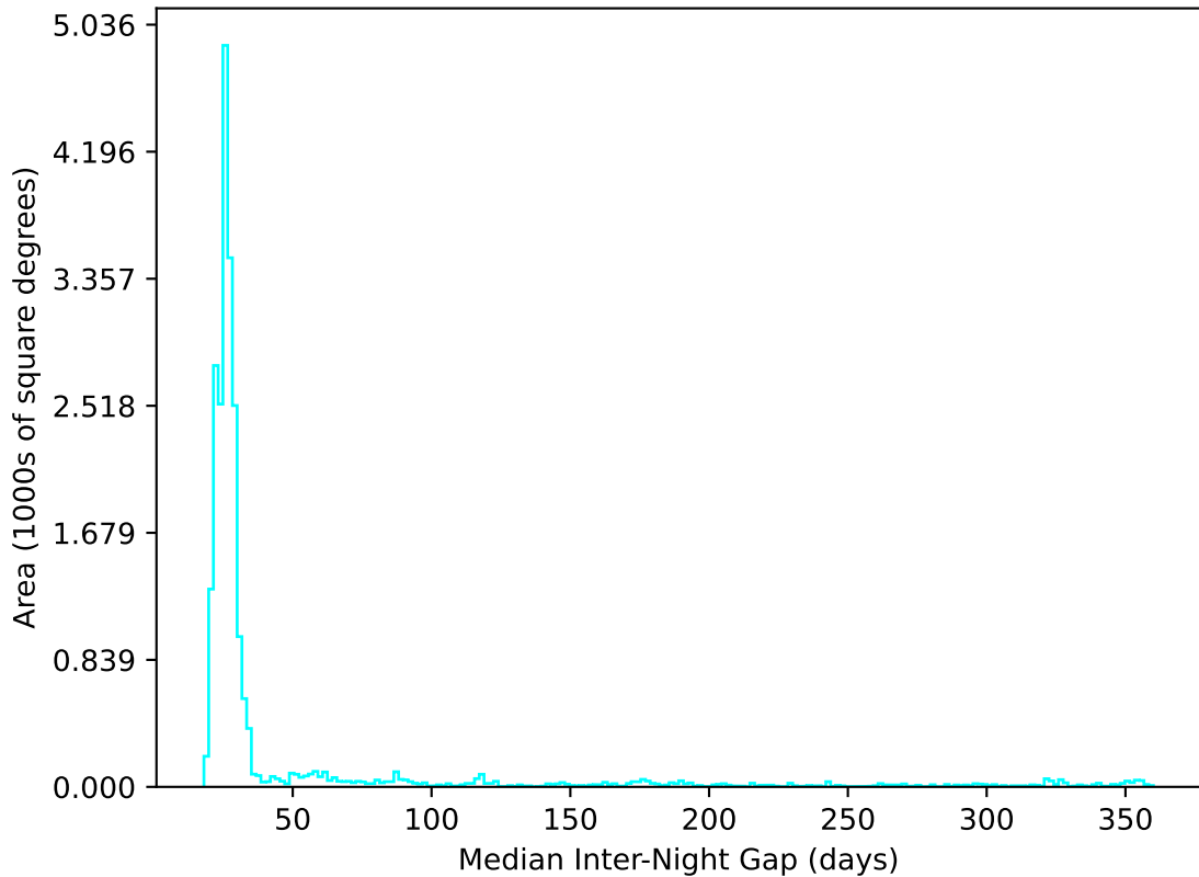
too_elab_r16_d3_ugrizy_v3.4_10yrs All sky u band: Median Inter-Night Gap
