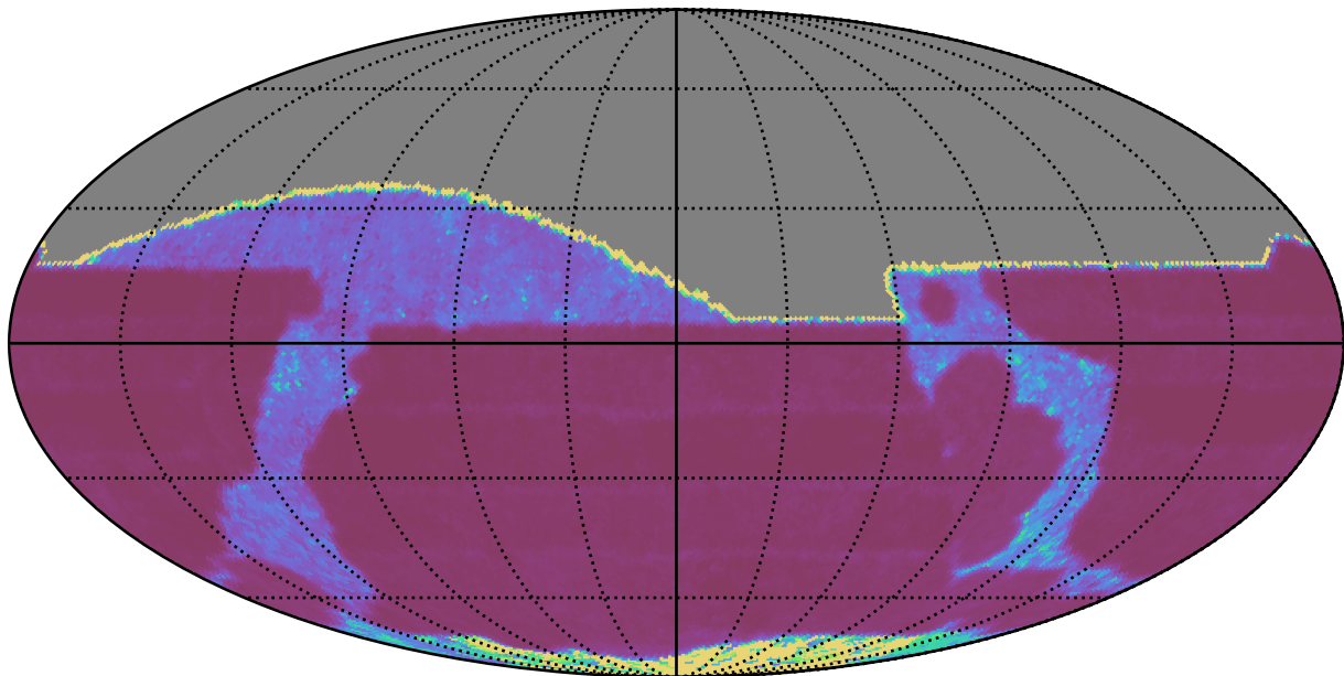
too_elab_r16_d3_ugrizy_v3.4_10yrs All sky r band: Median Inter-Night Gap
