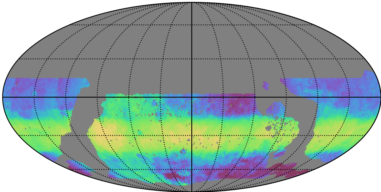
too_elab_r16_d3_ugrizy_v3.4_10yrs WFD z band: Median HA
