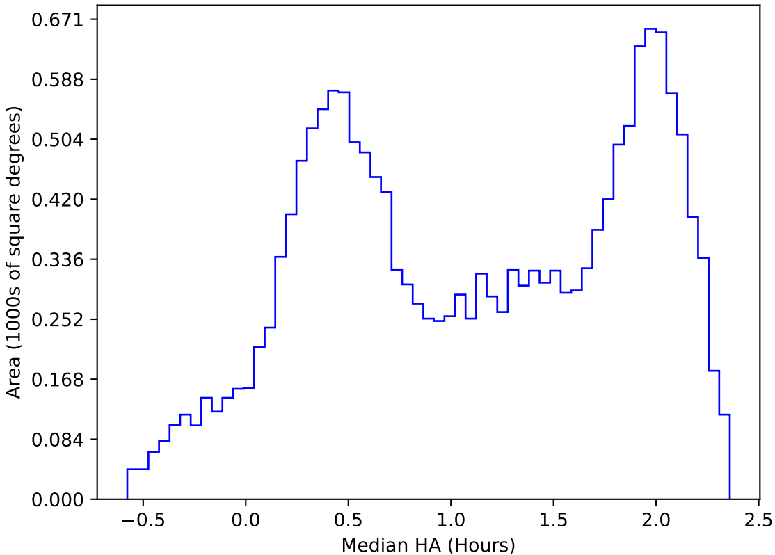
too_elab_r16_d3_ugrizy_v3.4_10yrs WFD z band: Median HA
