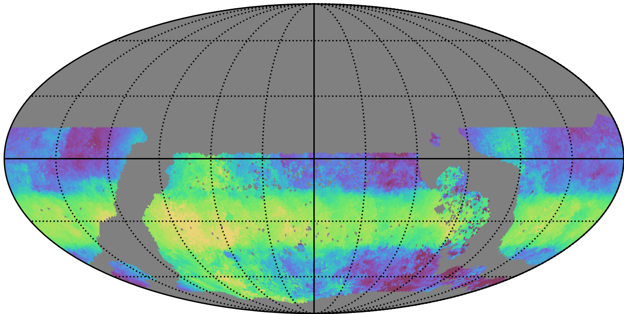
too_elab_r16_d3_ugrizy_v3.4_10yrs WFD u band: Median HA
