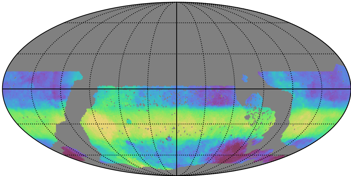
too_elab_r16_d3_ugrizy_v3.4_10yrs WFD r band: Median HA
