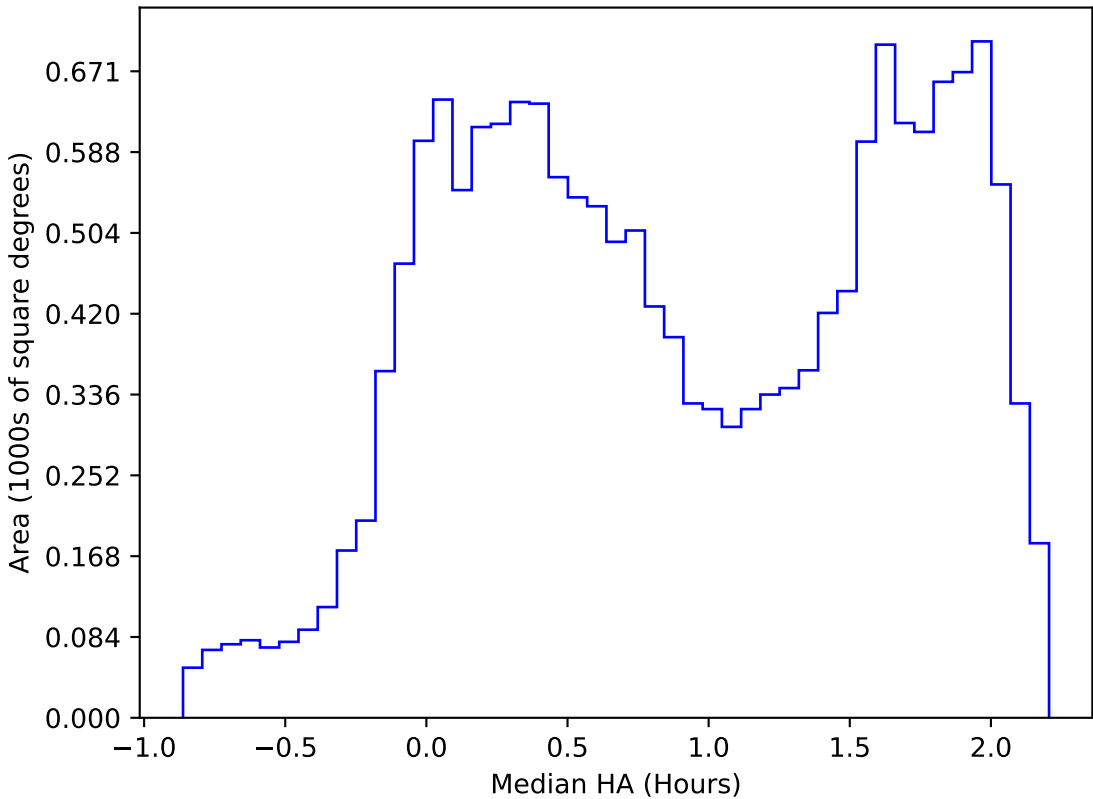
too_elab_r16_d3_ugrizy_v3.4_10yrs WFD r band: Median HA
