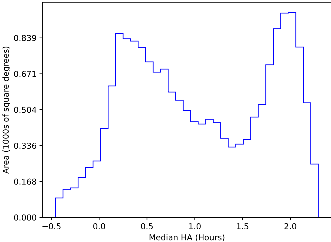
too_elab_r16_d3_ugrizy_v3.4_10yrs WFD i band: Median HA
