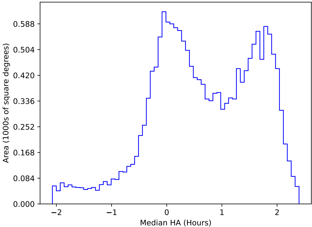
too_elab_r16_d3_ugrizy_v3.4_10yrs WFD g band: Median HA
