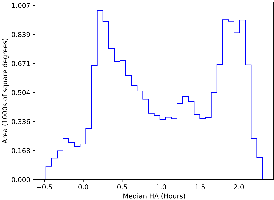
too_elab_r16_d3_ugrizy_v3.4_10yrs WFD all bands: Median HA
