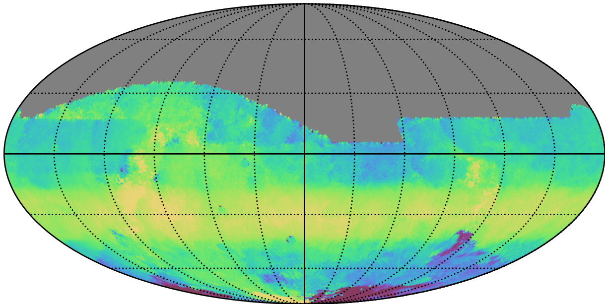
too_elab_r16_d3_ugrizy_v3.4_10yrs All sky z band: Median HA
