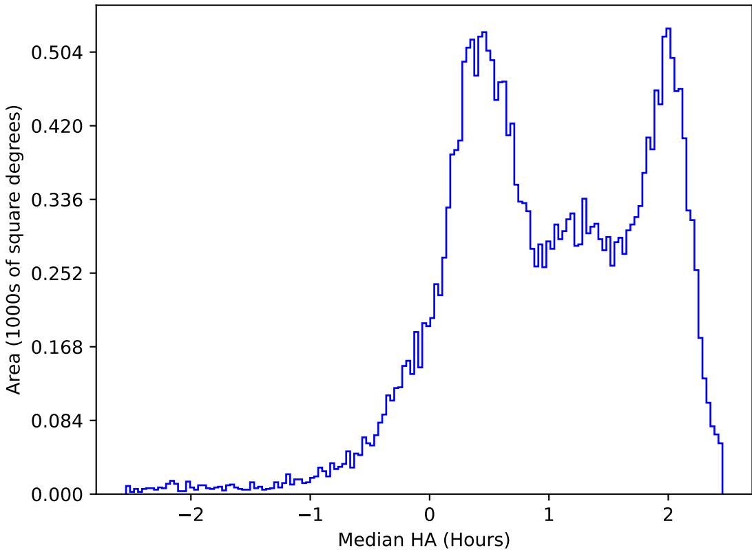
too_elab_r16_d3_ugrizy_v3.4_10yrs All sky z band: Median HA
