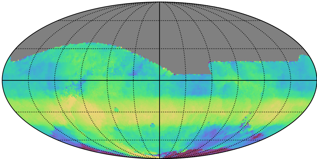
too_elab_r16_d3_ugrizy_v3.4_10yrs All sky r band: Median HA
