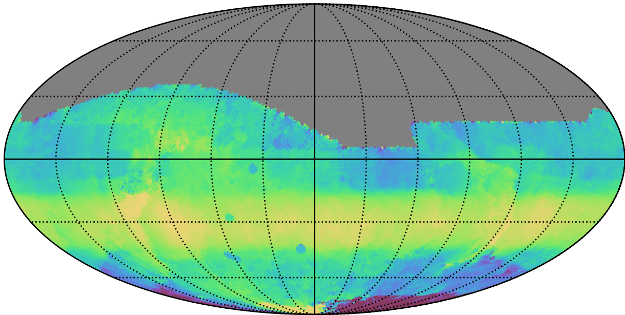
too_elab_r16_d3_ugrizy_v3.4_10yrs All sky i band: Median HA
