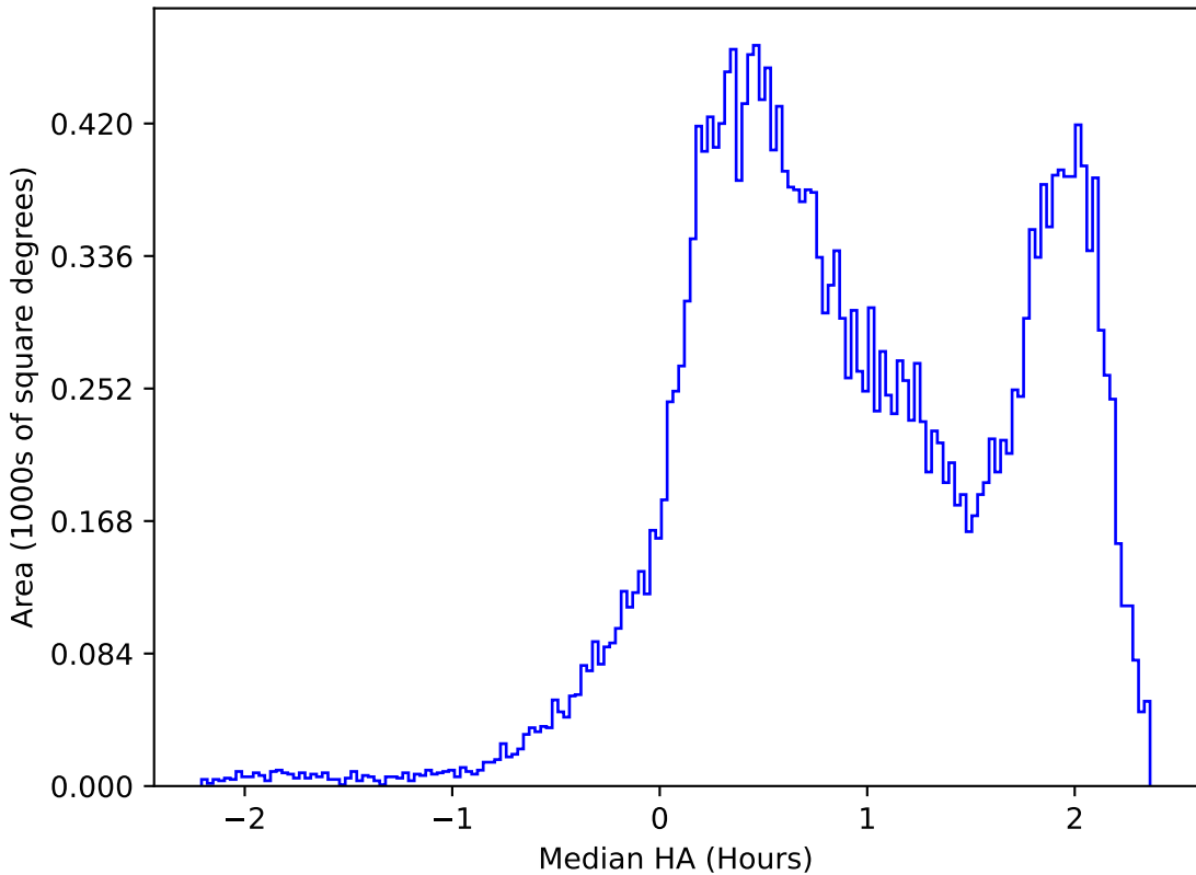
too_elab_r16_d3_ugrizy_v3.4_10yrs All sky i band: Median HA
