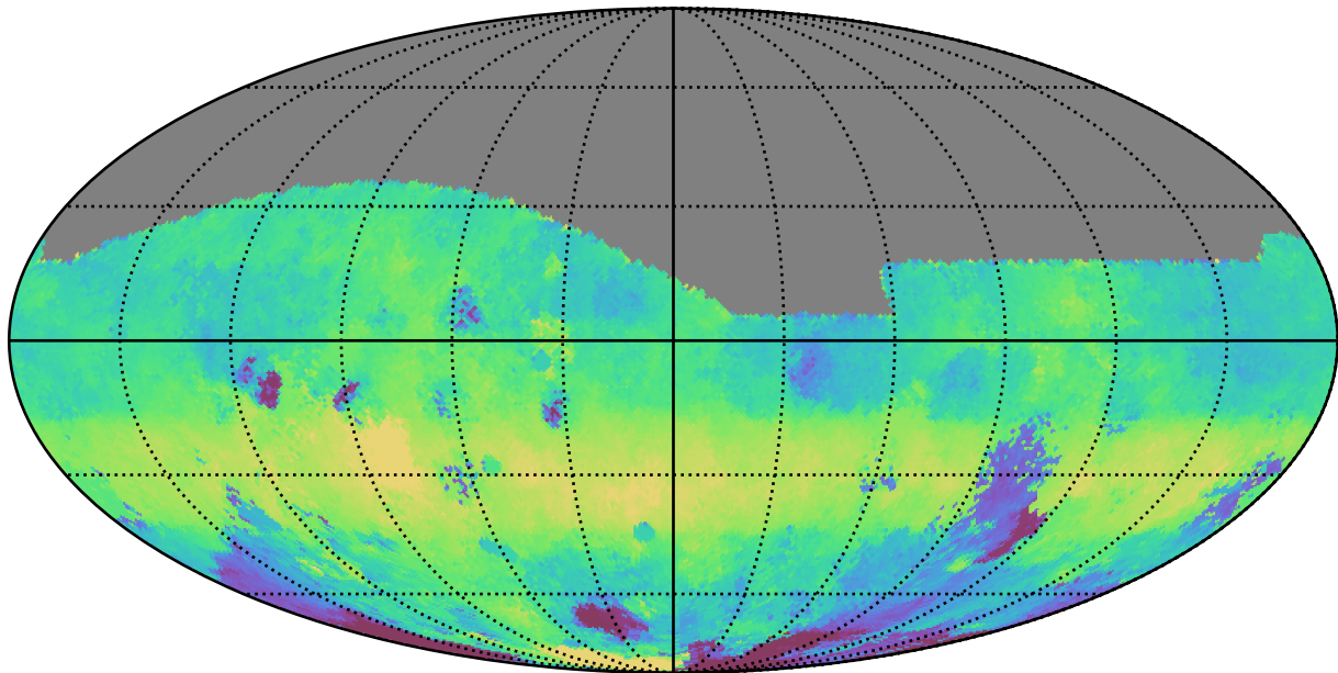
too_elab_r16_d3_ugrizy_v3.4_10yrs All sky g band: Median HA
