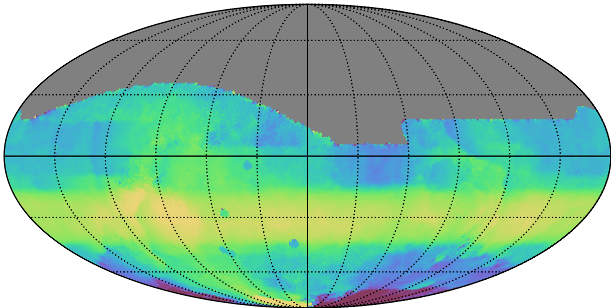
too_elab_r16_d3_ugrizy_v3.4_10yrs All sky all bands: Median HA
