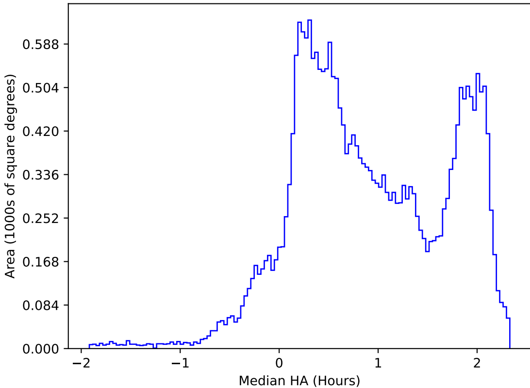
too_elab_r16_d3_ugrizy_v3.4_10yrs All sky all bands: Median HA
