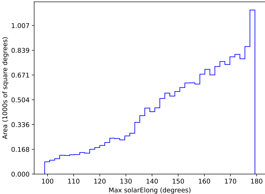
too_elab_r16_d3_ugrizy_v3.4_10yrs WFD r band: Max solarElong
