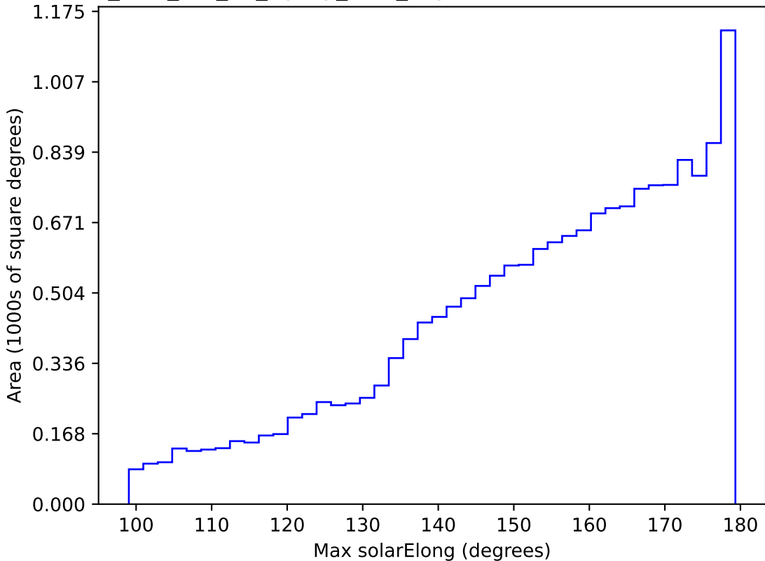
too_elab_r16_d3_ugrizy_v3.4_10yrs WFD i band: Max solarElong
