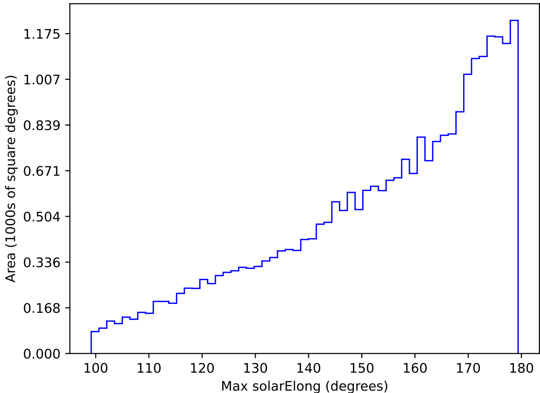
too_elab_r16_d3_ugrizy_v3.4_10yrs All sky z band: Max solarElong
