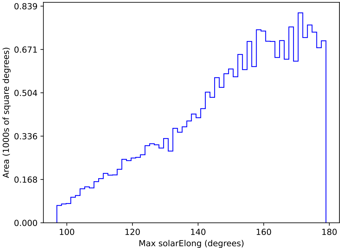
too_elab_r16_d3_ugrizy_v3.4_10yrs All sky u band: Max solarElong
