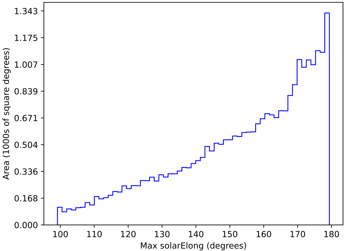
too_elab_r16_d3_ugrizy_v3.4_10yrs All sky r band: Max solarElong
