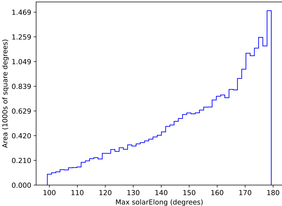
too_elab_r16_d3_ugrizy_v3.4_10yrs All sky i band: Max solarElong
