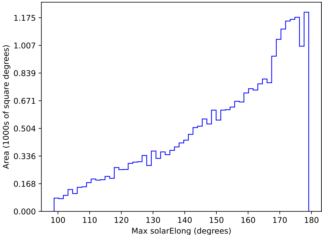
too_elab_r16_d3_ugrizy_v3.4_10yrs All sky g band: Max solarElong
