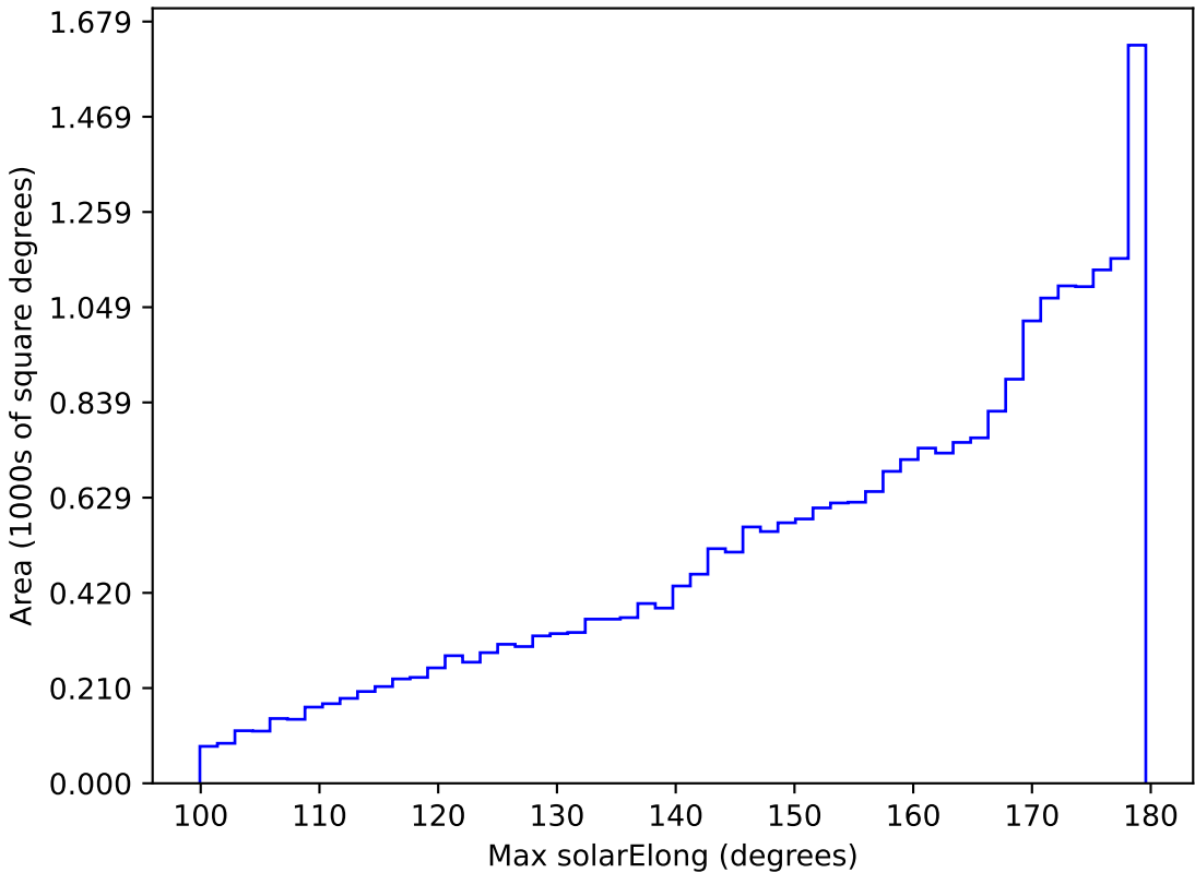
too_elab_r16_d3_ugrizy_v3.4_10yrs All sky all bands: Max solarElong
