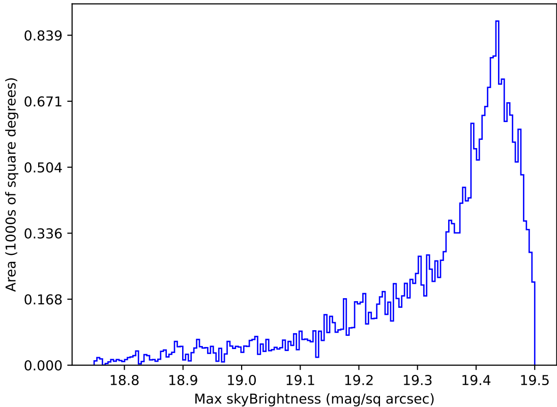
too_elab_r16_d3_ugrizy_v3.4_10yrs Yr 1 z band: Max skyBrightness
