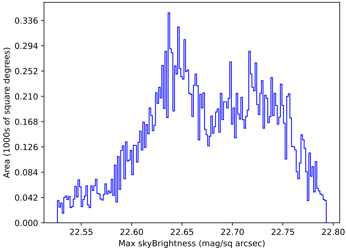
too_elab_r16_d3_ugrizy_v3.4_10yrs Yr 1 u band: Max skyBrightness
