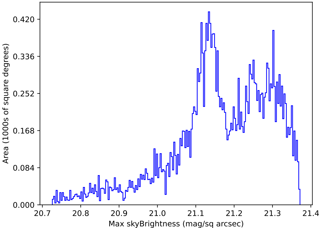
too_elab_r16_d3_ugrizy_v3.4_10yrs Yr 1 r band: Max skyBrightness
