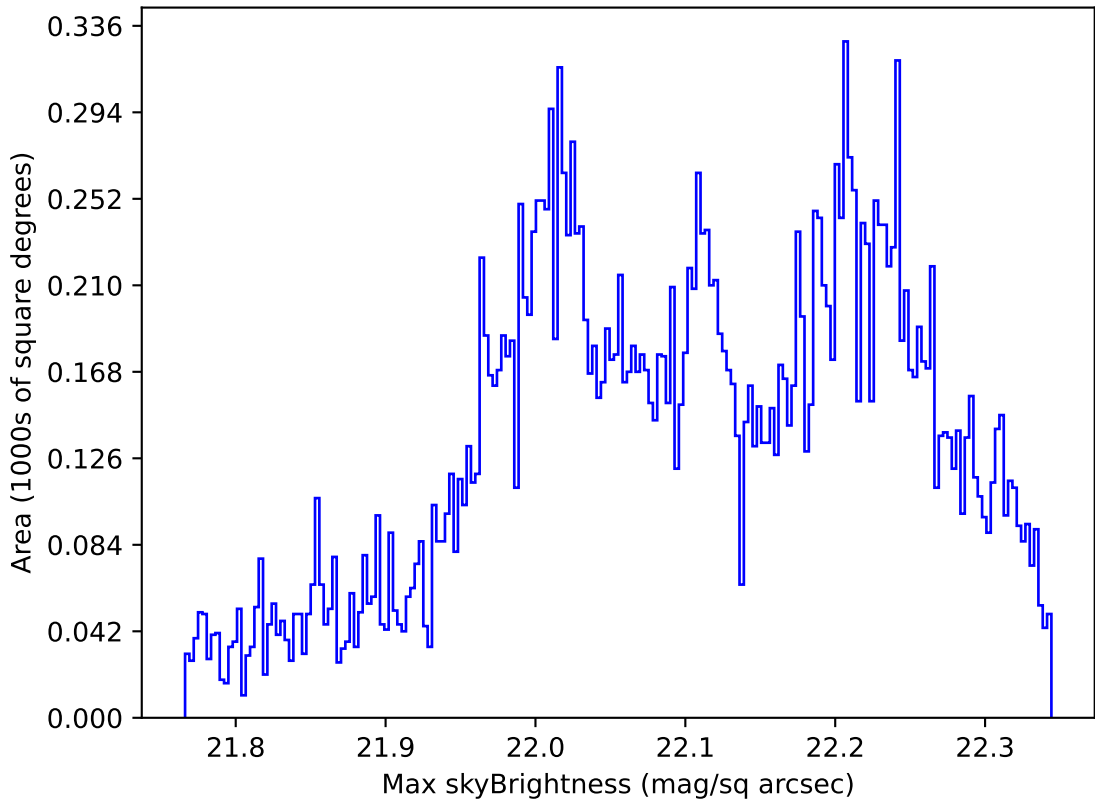
too_elab_r16_d3_ugrizy_v3.4_10yrs Yr 1 g band: Max skyBrightness
