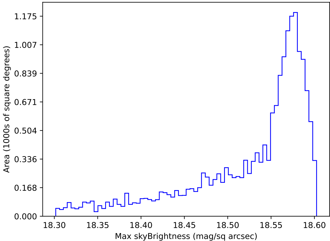
too_elab_r16_d3_ugrizy_v3.4_10yrs WFD y band: Max skyBrightness
