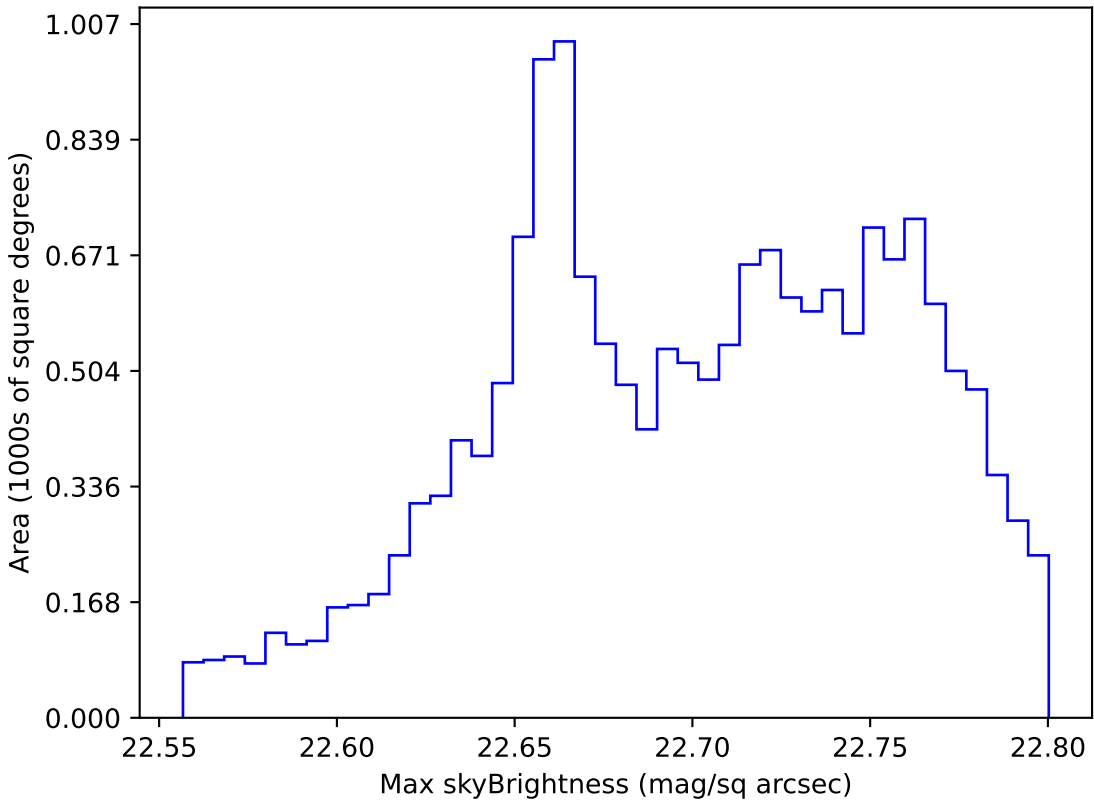
too_elab_r16_d3_ugrizy_v3.4_10yrs WFD u band: Max skyBrightness
