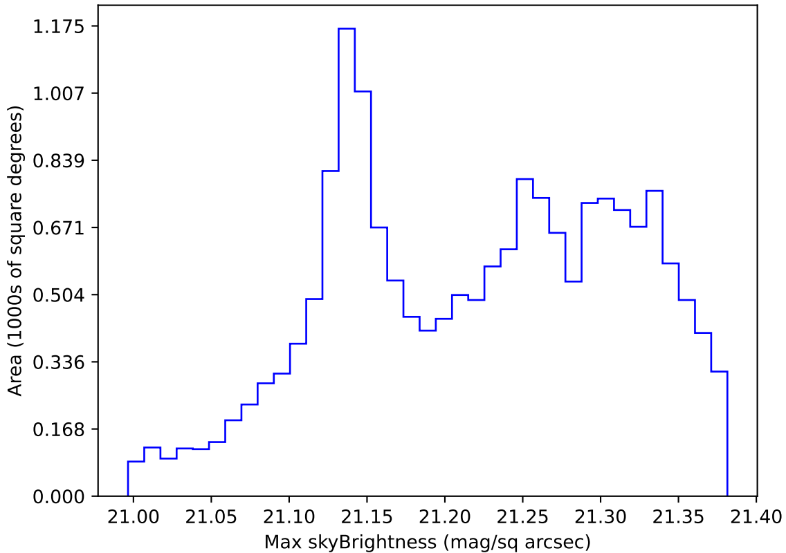
too_elab_r16_d3_ugrizy_v3.4_10yrs WFD r band: Max skyBrightness
