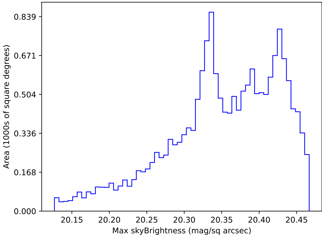
too_elab_r16_d3_ugrizy_v3.4_10yrs WFD i band: Max skyBrightness
