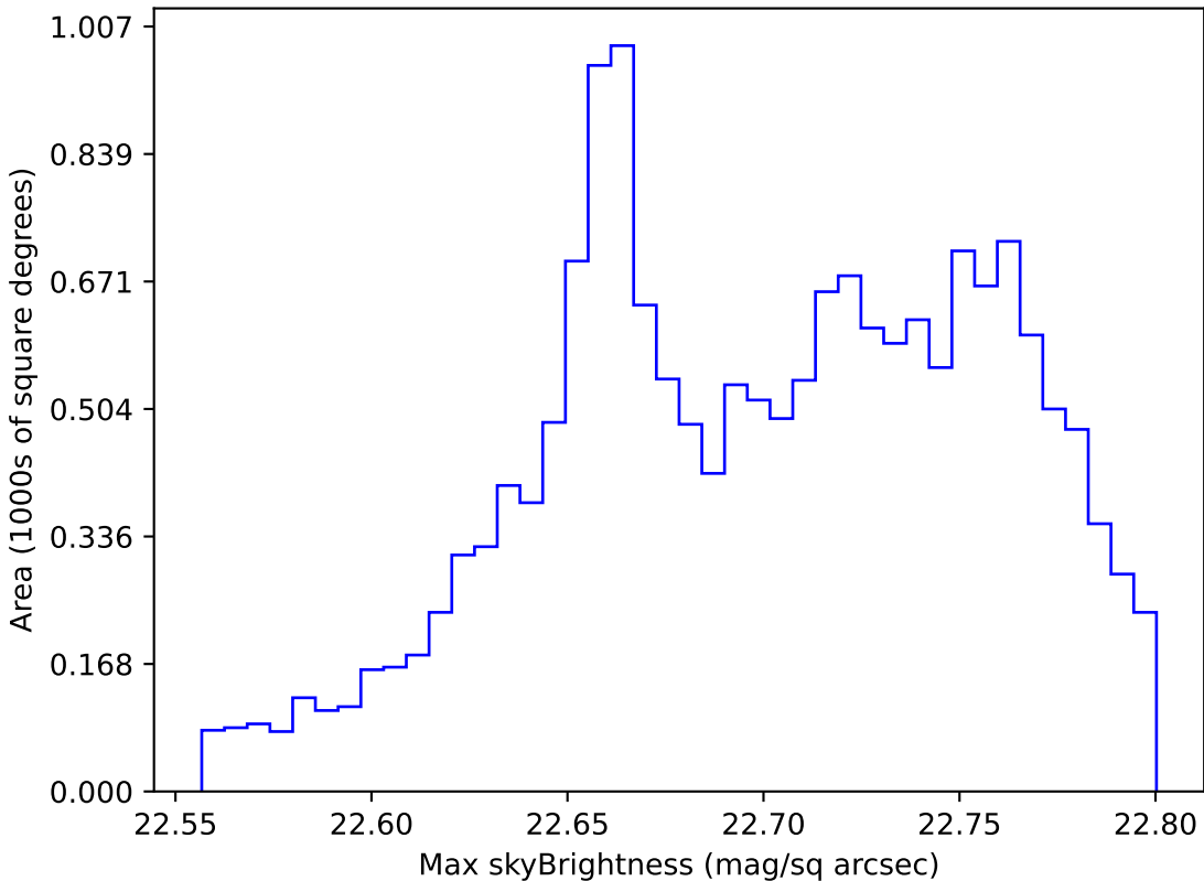
too_elab_r16_d3_ugrizy_v3.4_10yrs WFD all bands: Max skyBrightness
