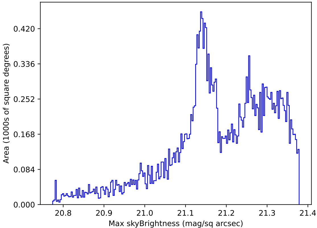
too_elab_r16_d3_ugrizy_v3.4_10yrs All sky r band: Max skyBrightness
