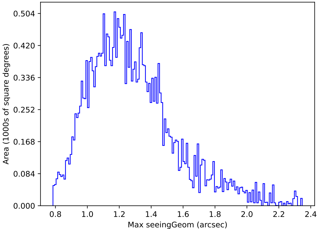
too_elab_r16_d3_ugrizy_v3.4_10yrs Yr 1 z band: Max seeingGeom
