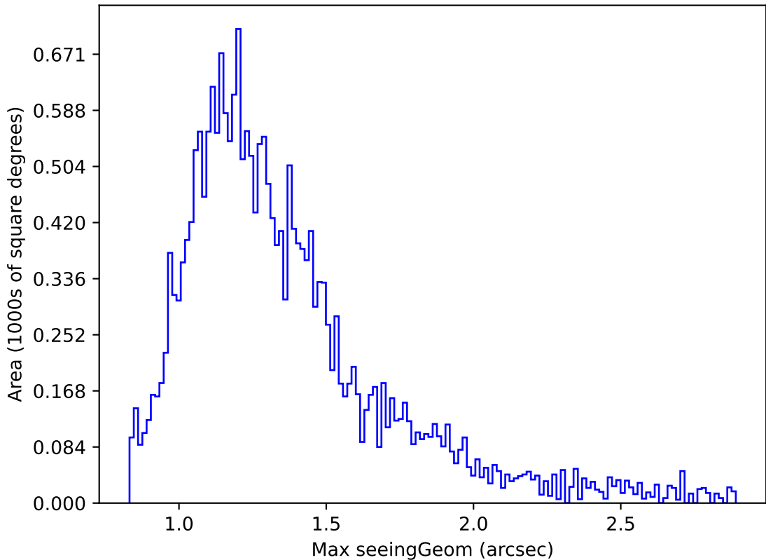
too_elab_r16_d3_ugrizy_v3.4_10yrs Yr 1 u band: Max seeingGeom
