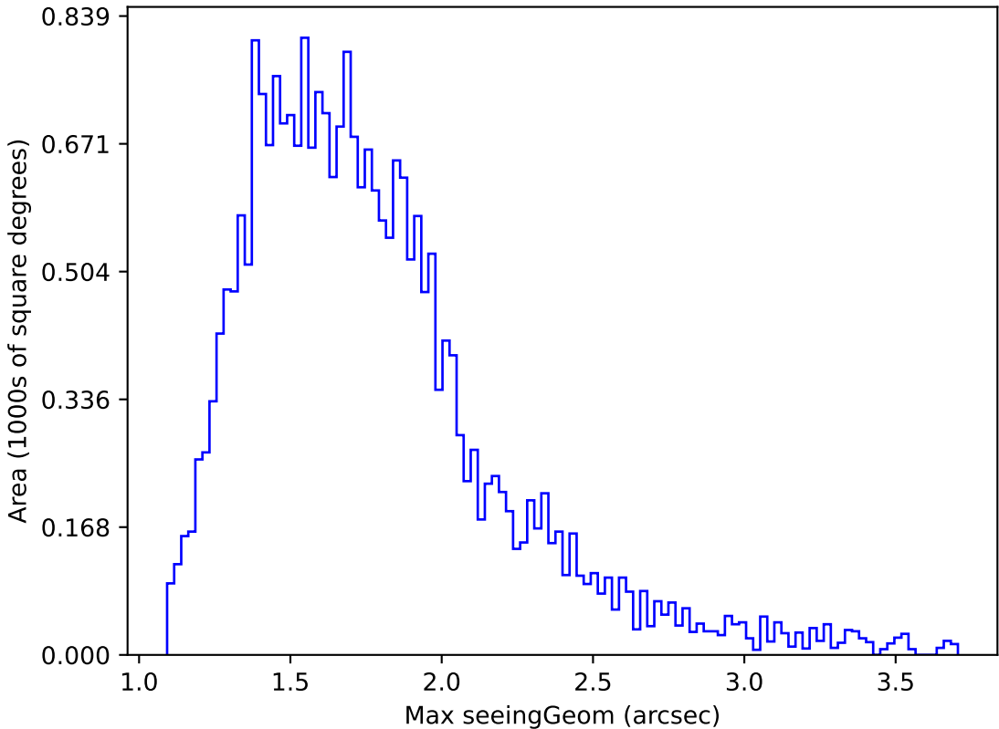
too_elab_r16_d3_ugrizy_v3.4_10yrs Yr 1 all bands: Max seeingGeom
