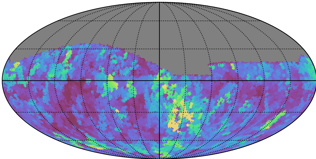
too_elab_r16_d3_ugrizy_v3.4_10yrs Yr 1 z band: Max seeingEff
