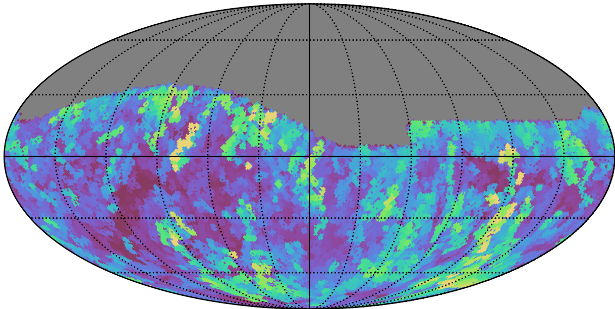
too_elab_r16_d3_ugrizy_v3.4_10yrs Yr 1 r band: Max seeingEff
