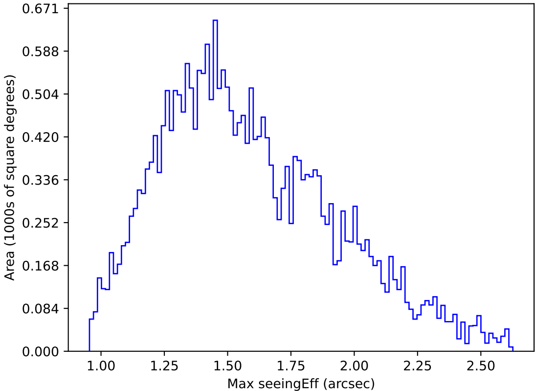
too_elab_r16_d3_ugrizy_v3.4_10yrs Yr 1 r band: Max seeingEff
